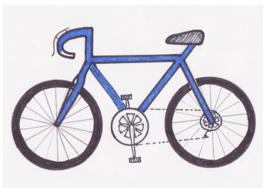
bike
