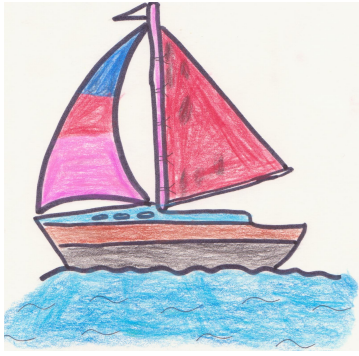
boat
