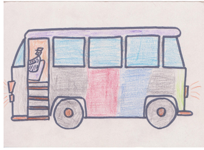
bus
