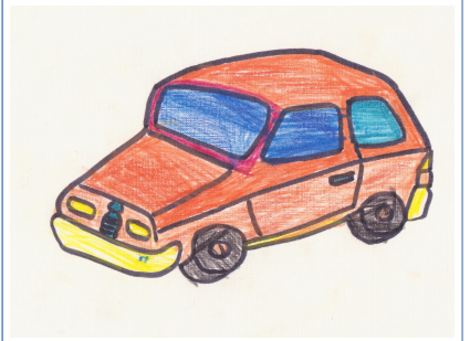
car
